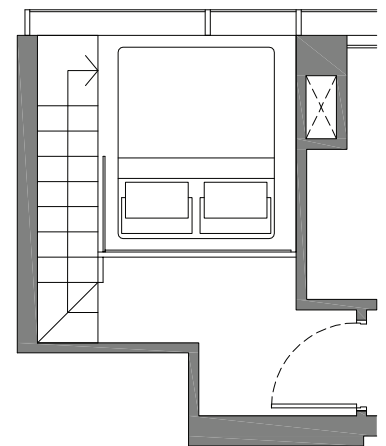
FURNITURE DECK
